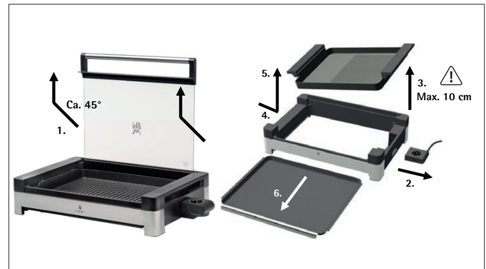
Fig. 2 - Demontage /Disassembling
