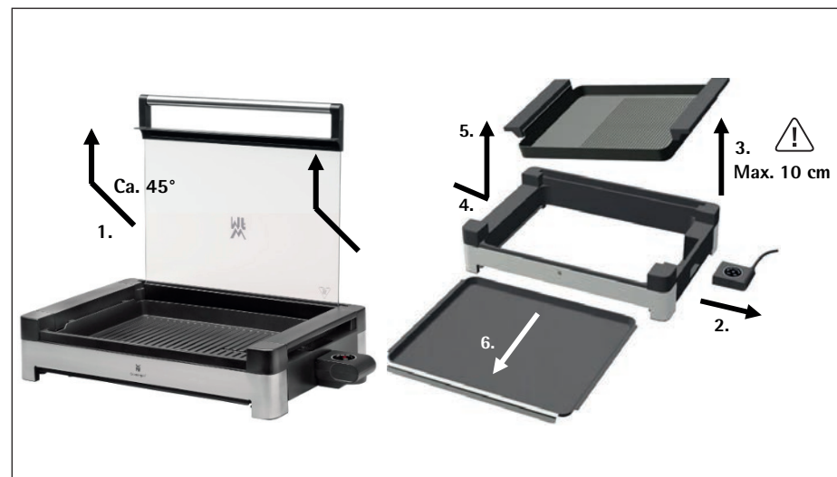
Fig. 2 - Demontage /Disassembling
