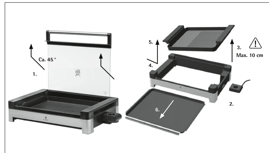
Fig. 2 - Demontage /Disassembling
