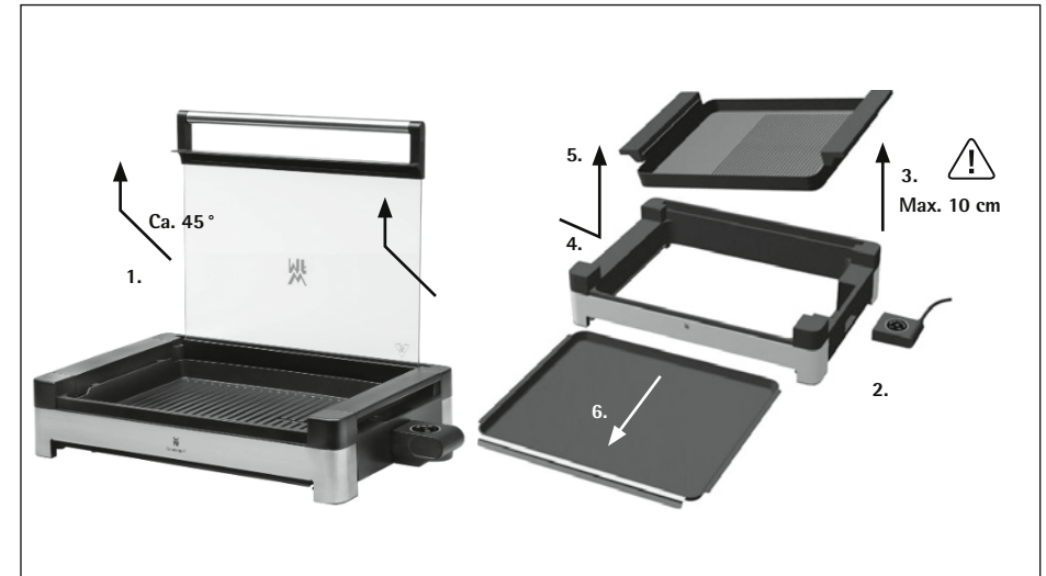
afb. 2 - Demontage /Disassembling
