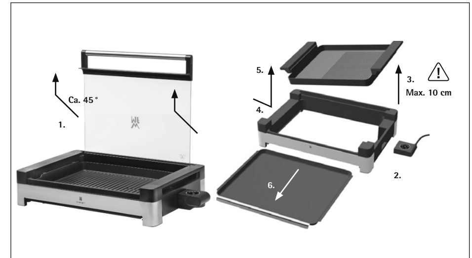
Abb. 2 - Demontage /Disassembling
